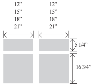
Opening Dimensions
