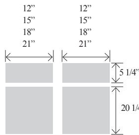
Opening Dimensions
