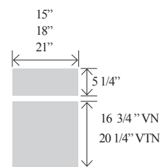
Opening Dimensions
