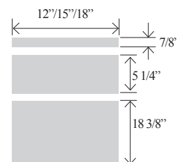
Opening Dimensions
