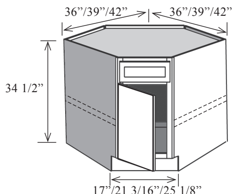
Opening dimensions
