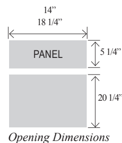
Opening Dimensions
