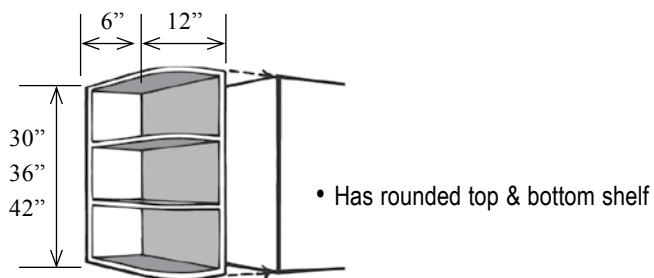
Quarter Round End Shelves
