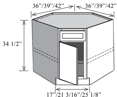
Opening dimensions
