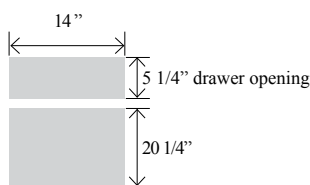
Opening dimensions
