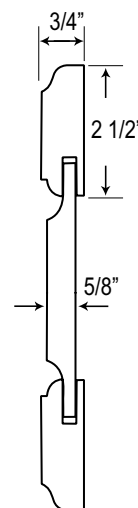
Raised Panel Door
