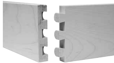
Drawer (2) 5/8" Thick Dovetail Solid Maple Wood Drawer Box
