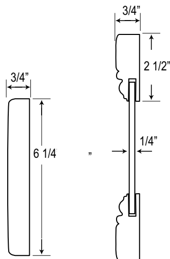
Solid Drawer Front
