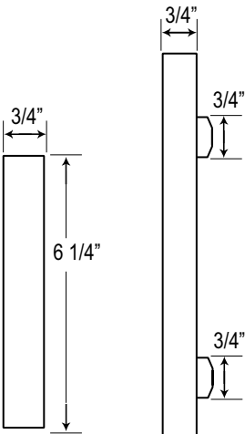
Solid Drawer Front
