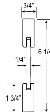
Flat Panel Mission Drawer Front
