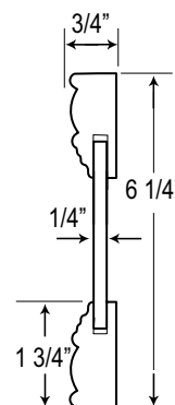
Flat Panel Mitered Drawer Front
