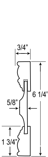
Raised Panel Mitered Drawer Front
